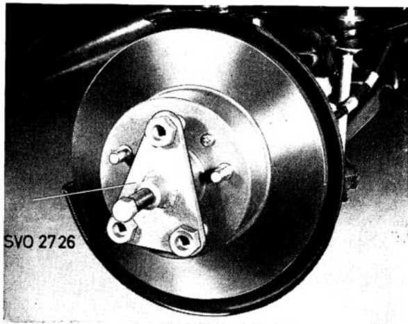
Fig. 7-20. Removing the hub
