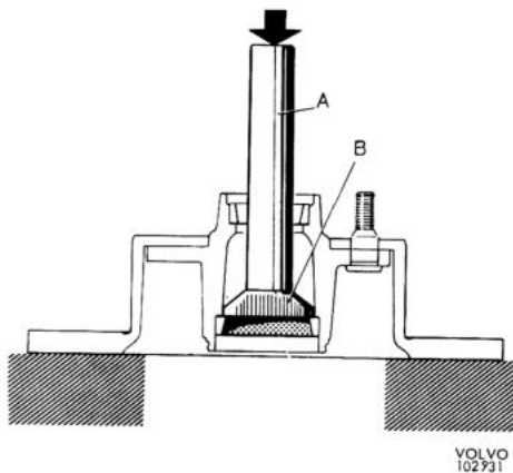
Fig. 7-22. Removing the inner bearing ring A = SVO 1801 B = SVO 2724
