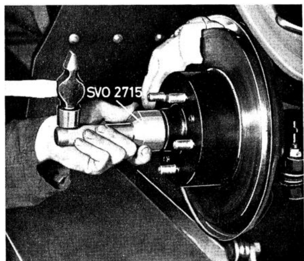
Fig. 7-19. Removing the grease cap
