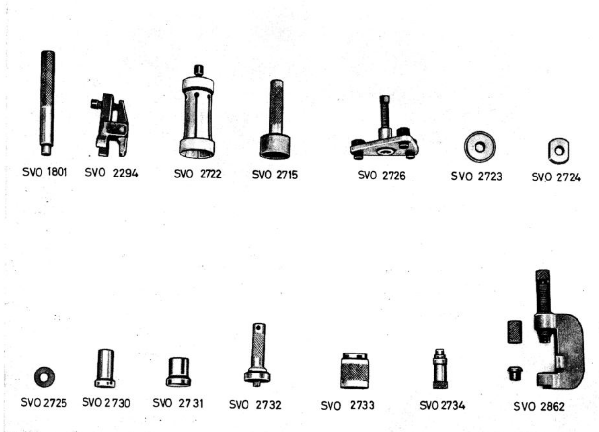
Fig. 7-1. Tools used for work on the rear axle suspension and hub
