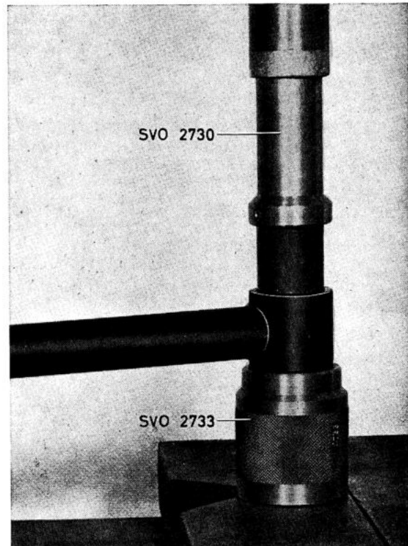
Fig. 7-12. Fitting the small bush, track bar
