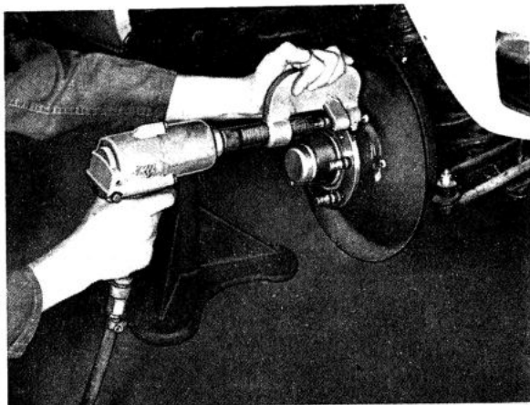
Fig. 7-17. Removing the wheel stud
