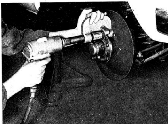
Fig. 7-18. Fitting the wheel stud
