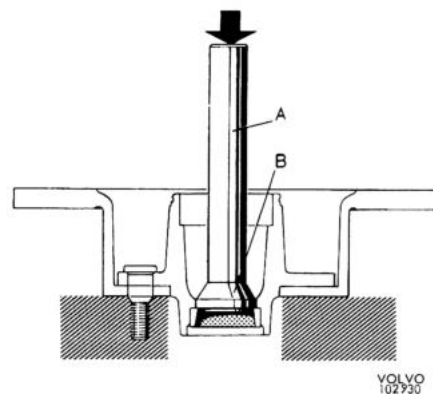
Fig. 7-23. Removing the outer bearing ring A = SVO 1801 B = SVO 2725
