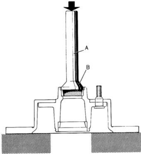
Fig. 7-25. Fitting the outer bearing ring A = SVO 1801 B = SVO 2724
