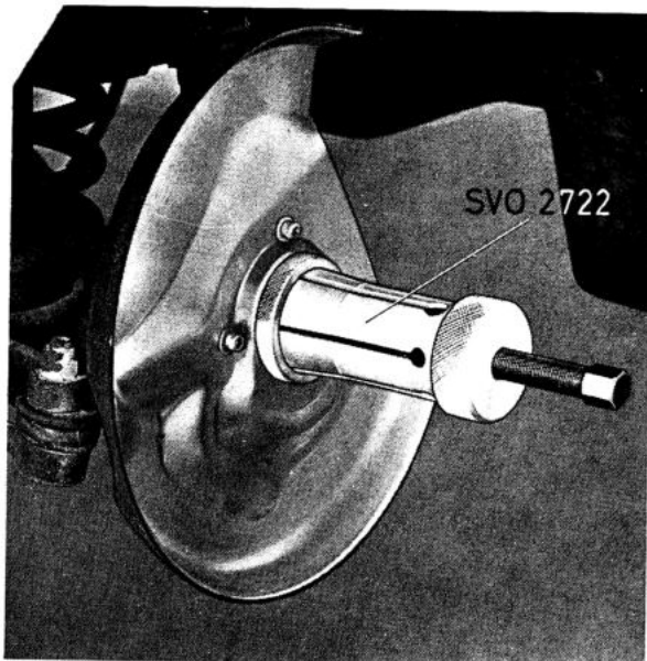
Fig. 7-21. Removing the inner bearing
