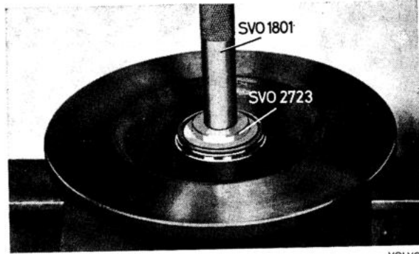
Fig. 7-26. Fitting the seal
