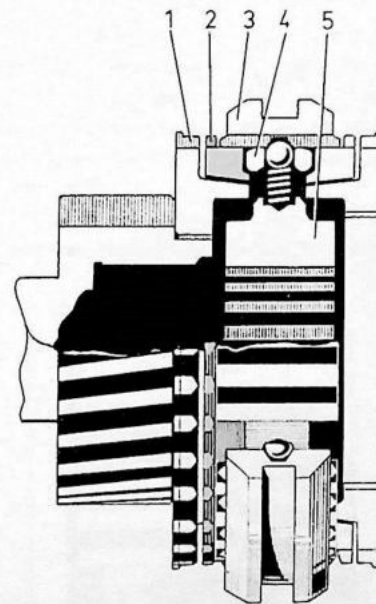
Afb. 3. Neutrale stand
