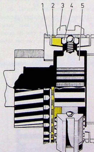
Afb. 3. Neutrale stand
