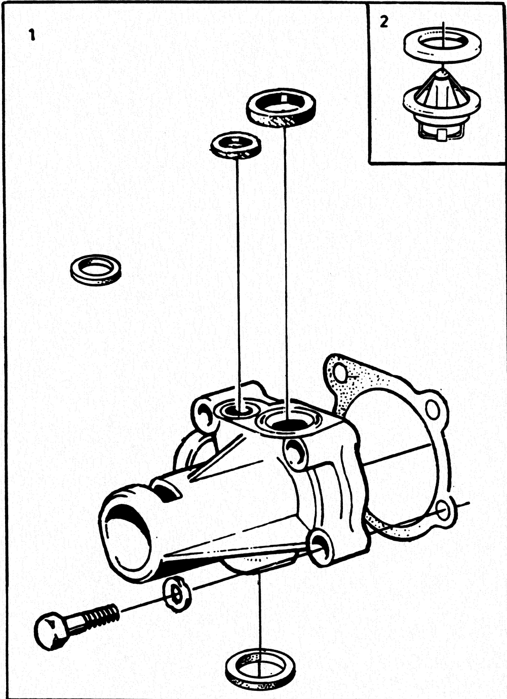
(111:1) VOLVO PARTS 1 101 20883
