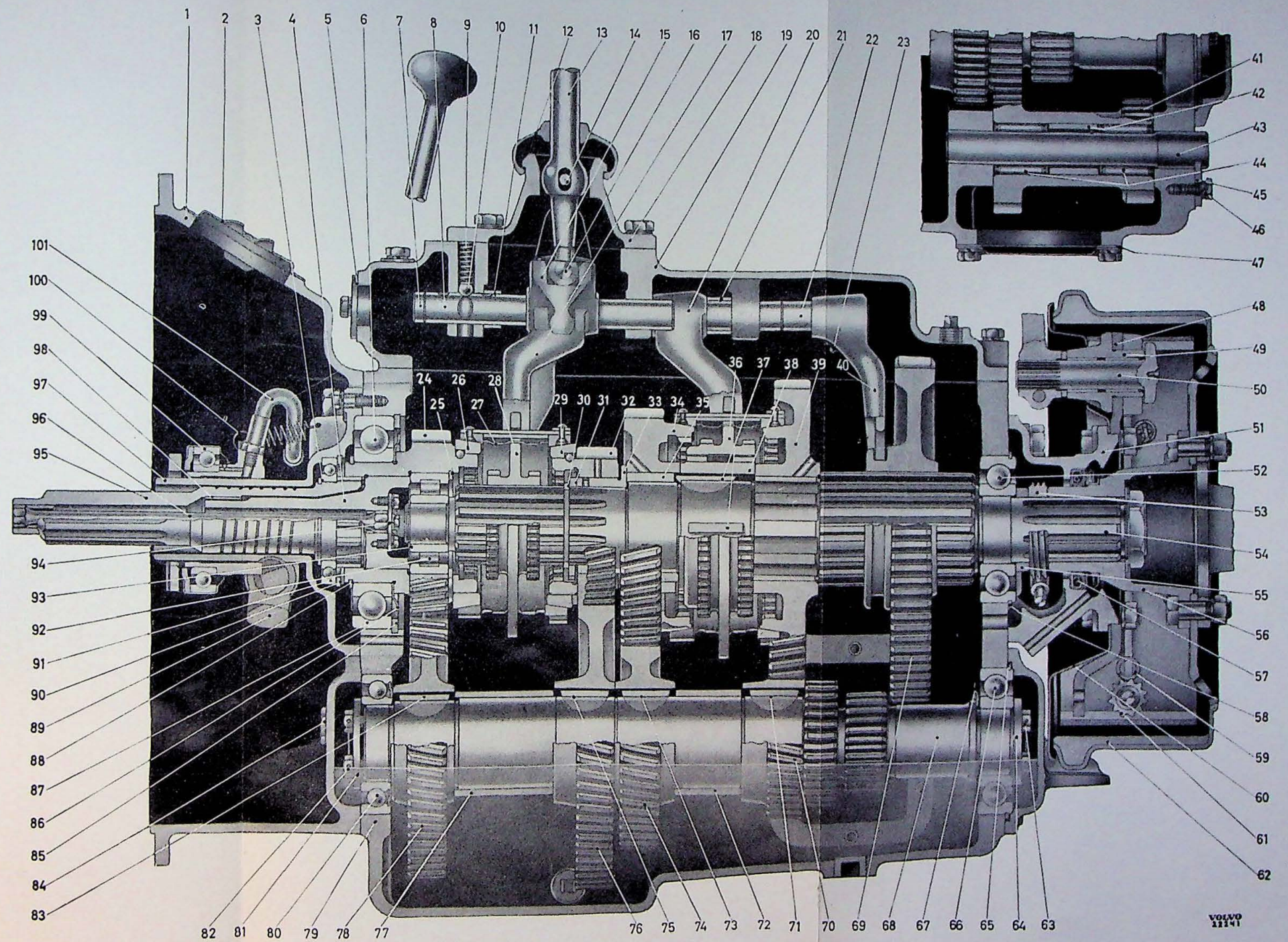
Illustration 3-A Type K 12, K 13 Transmission
