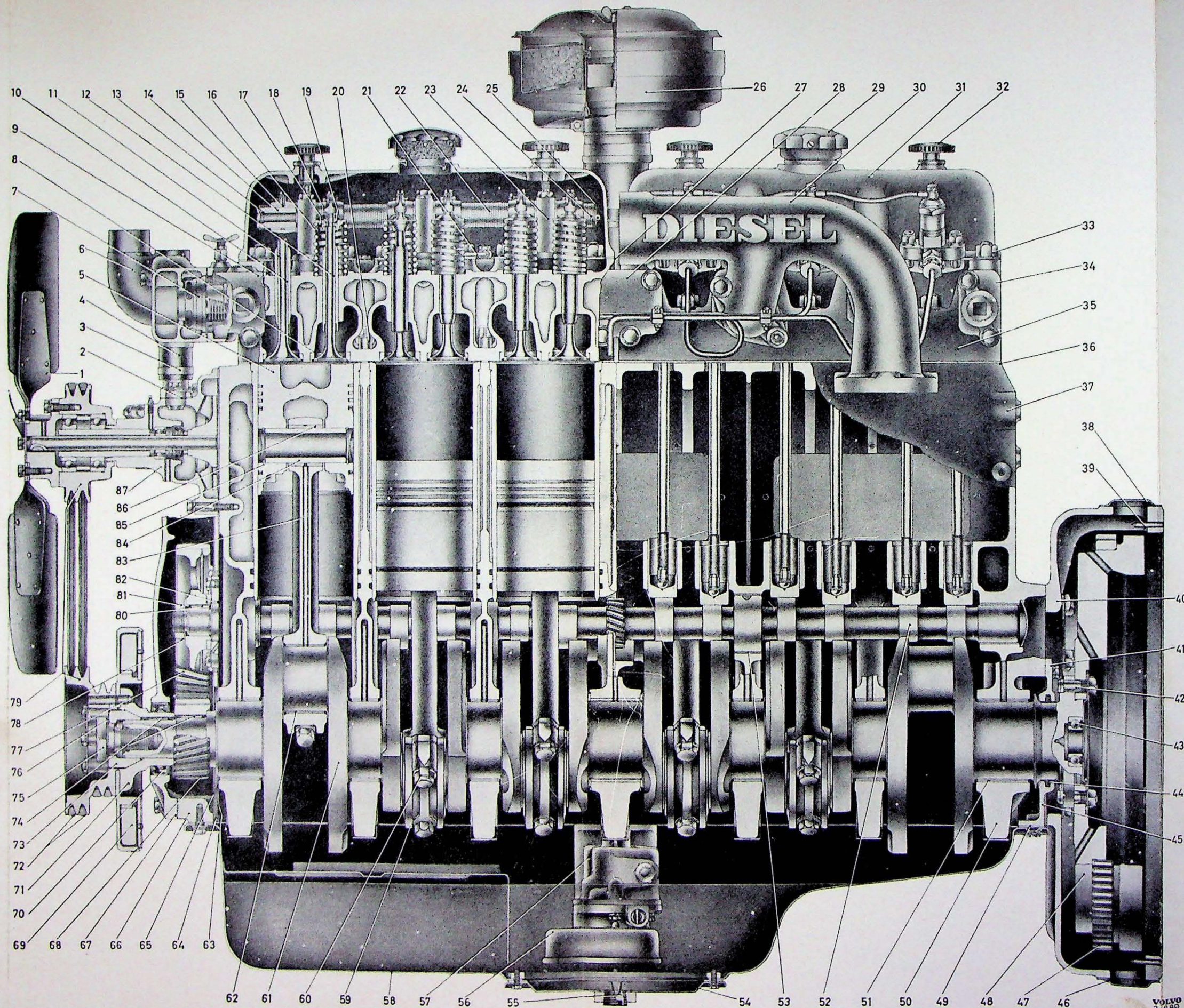
Illustration 1-A. D 67 A Diesel engine, longitudinal section
