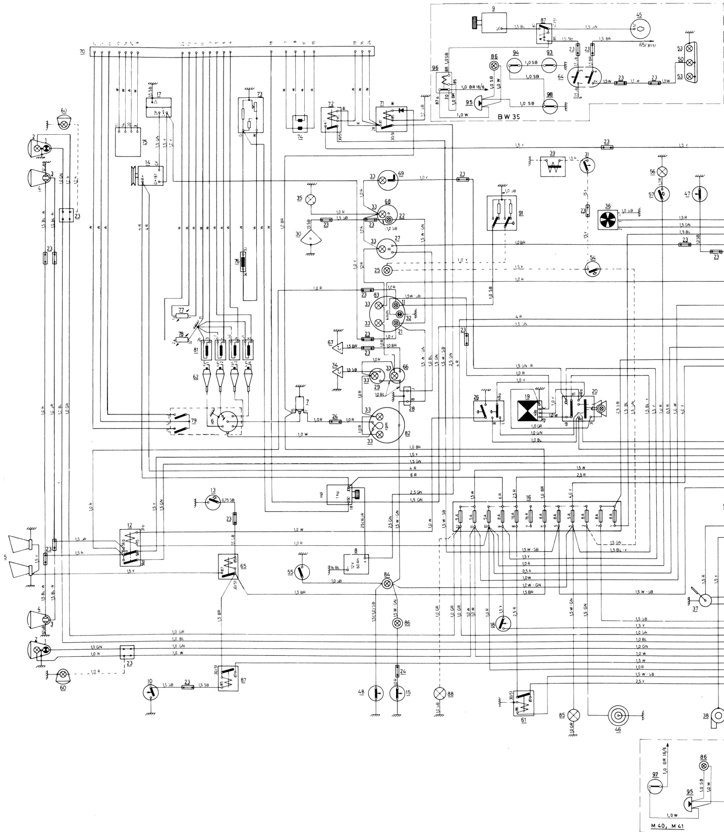
ILLUSTRATION 3-A. WIRING DIAGRAM 1800 E
