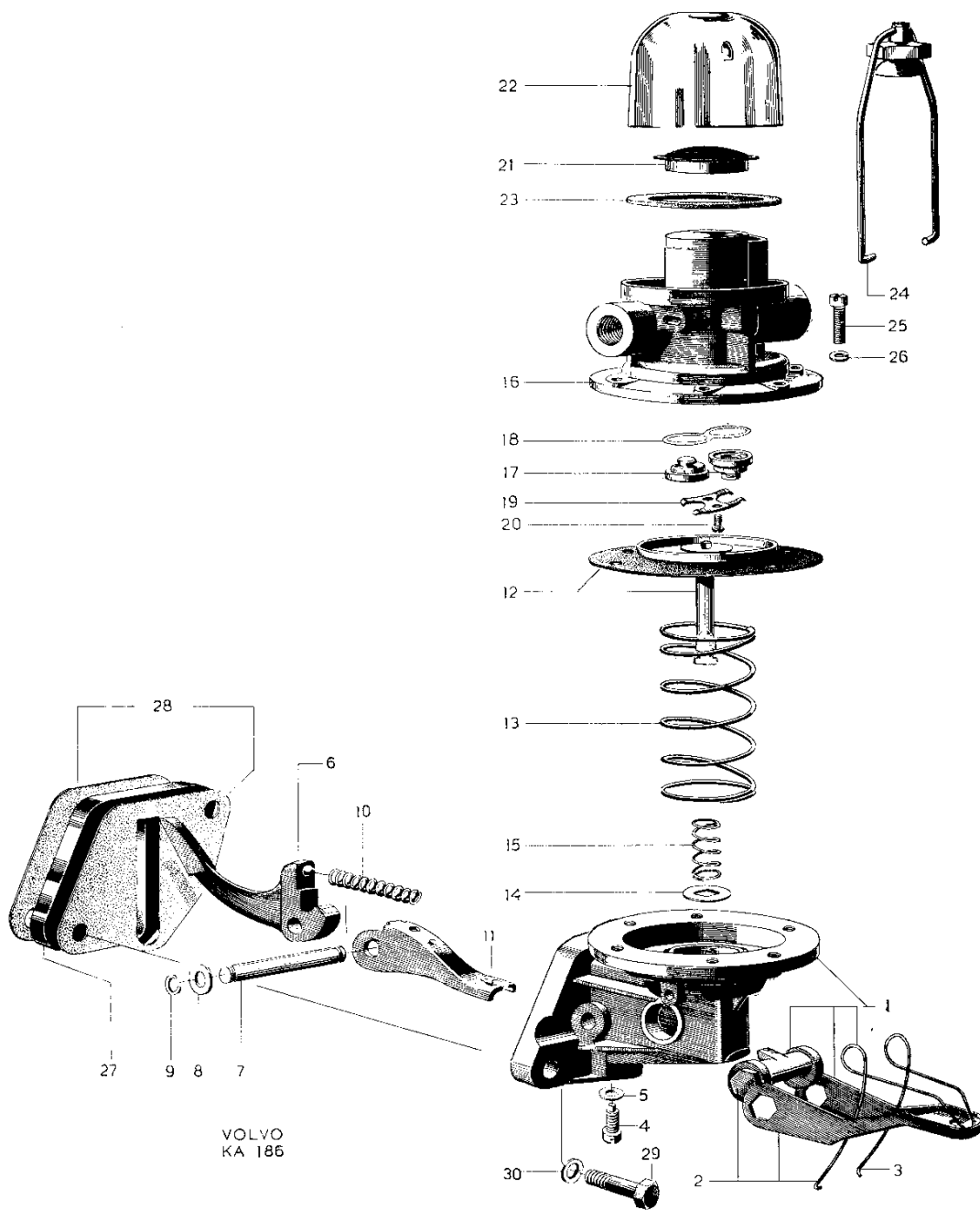
Fig. 7. Fuel pump
