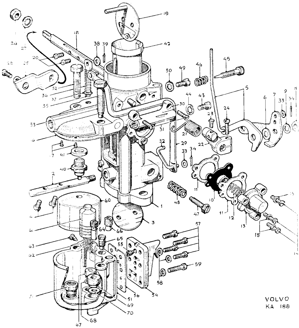
Fig. 9. Carburettor, Part Nos. 71670 and 71860
