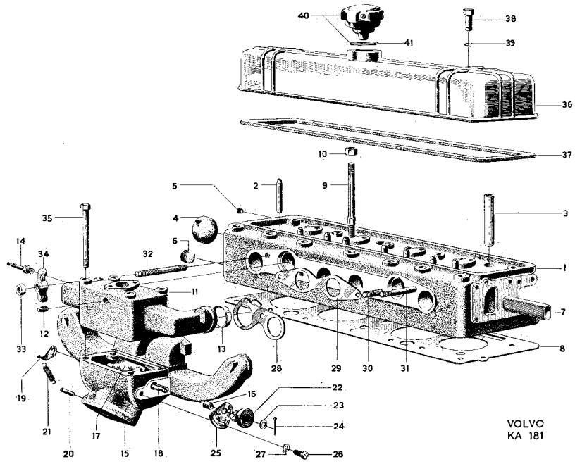
Fig. 2. Cylinder head and appurtenant parts
