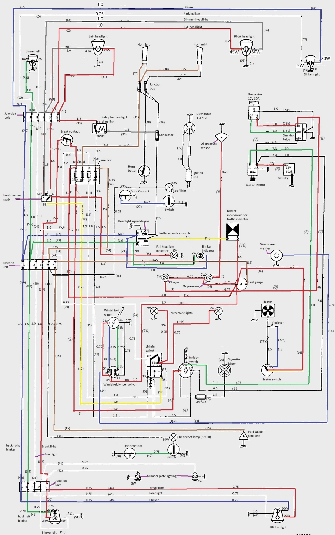
Wiring diagram PV 544 w.e.fr. chassis No. 330100 P 210 w.e.fr. chassis No. 51935
